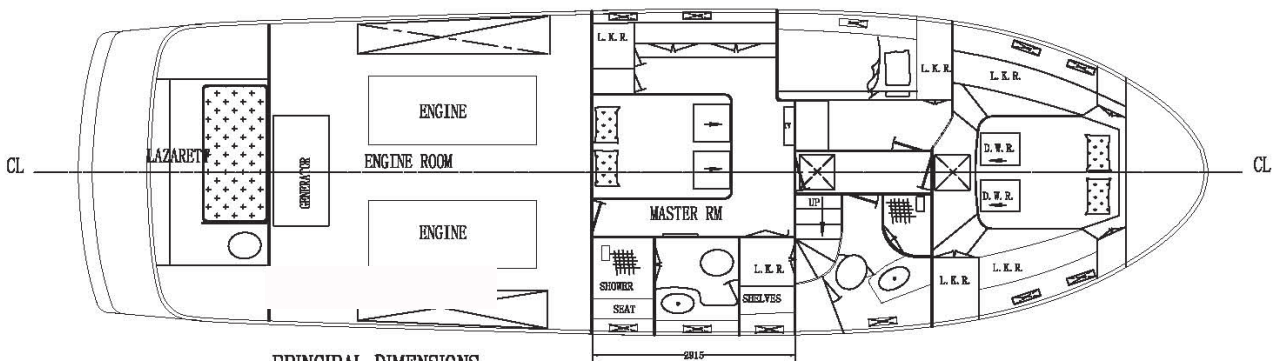
PRINCIPAL DIMENSIONS
